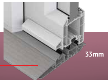
ALUMINIUM LOW THRESHOLD AND TRAY RAMP
