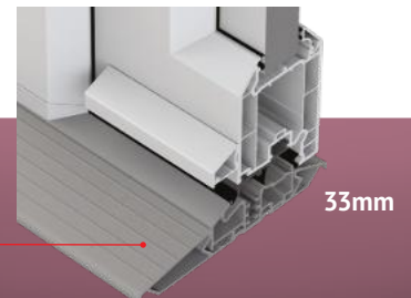
ALUMINIUM LOW THRESHOLD AND TRAY RAMP
